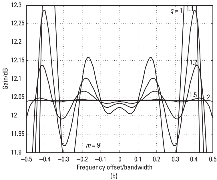
Figure 6.10 Sum beam frequency response; variation with equalization parameters: (a) variation with m ; and (b) variation with q .
