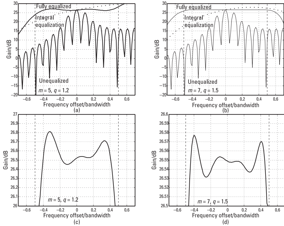
Figure 6.16 Difference beam slope: (a) small filter response; (b) larger filter response; (c) expanded small filter response; (d) expanded larger filter response.
