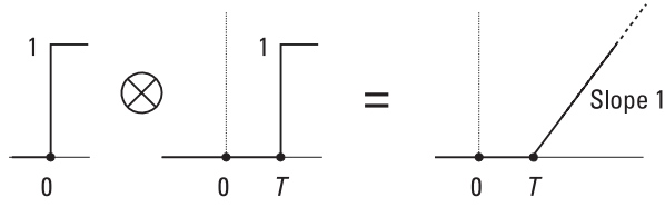
Figure 3.15 Ramp function.
